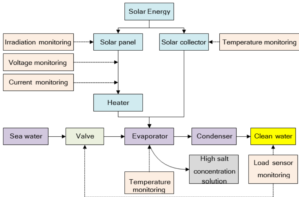
Figure 1. Seawater distillation proposed system.
